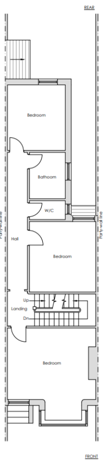
Existing First Floor Plan
